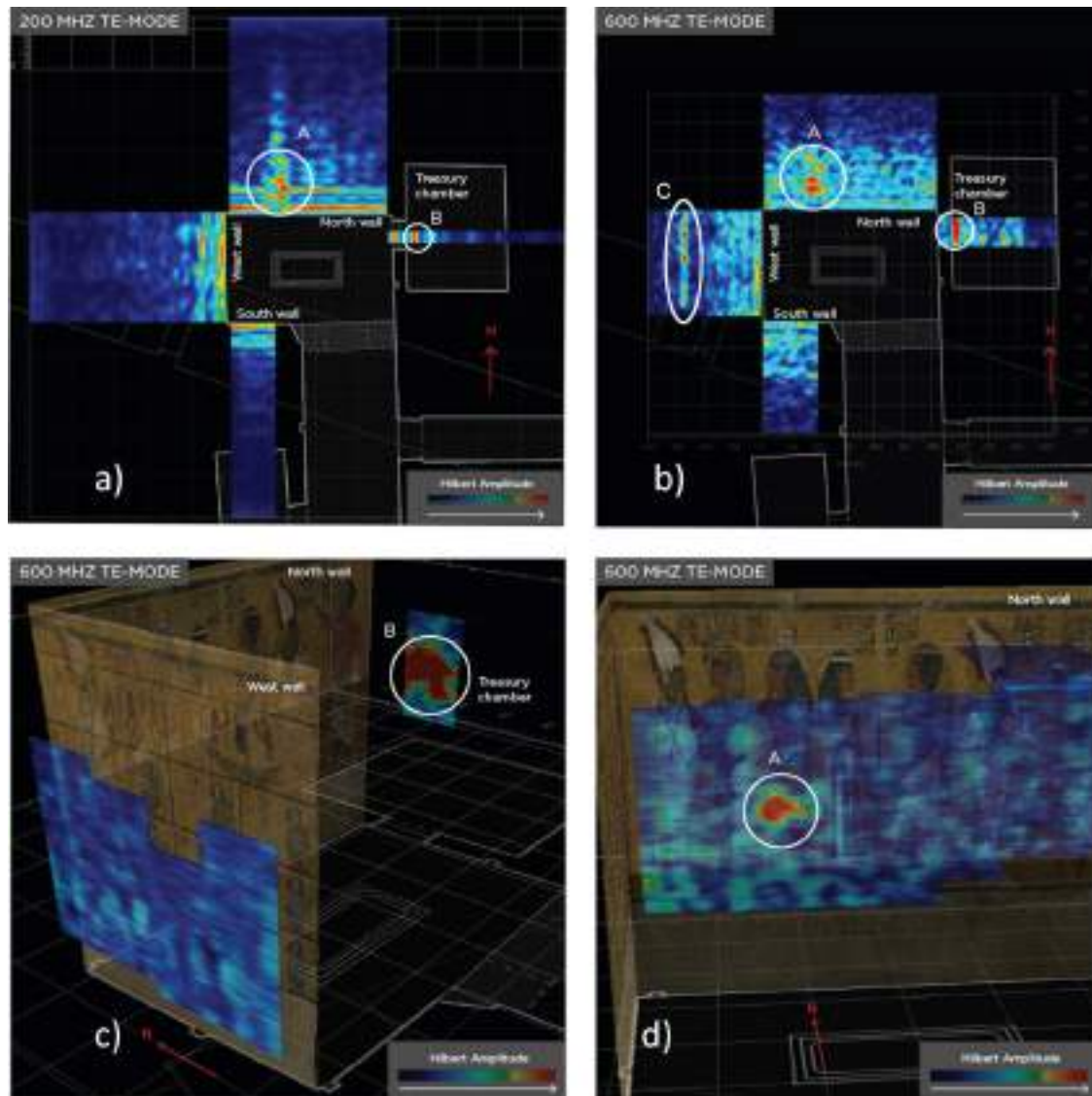
Fig. 5. IF and LF processed data: top view of representative horizontal cross sections for a: LF processed data and b: IF processed data, vertical cuts at 0.6 m depth from the IF GPR volume (TE-mode) behind the west c) and north wall d) are also reported. Evidence of: A wall repair anomaly, B wall separating the Burial Chamber from the Treasury Chamber and C deep linear reflection event are reported in all the panels.
