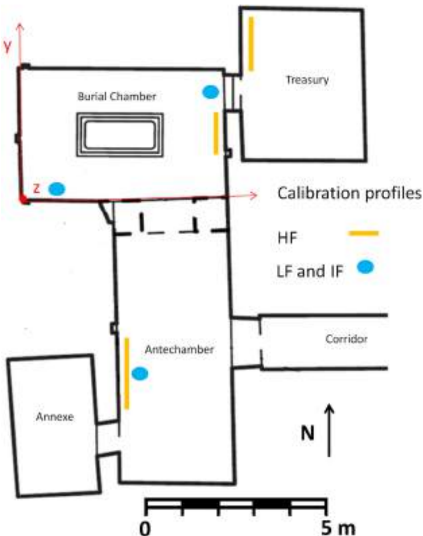
Fig. 1. plan view of the KV62 with indication of the reference system used for survey positioning and the location of the calibration profiles: yellow lines are the HF scans profiles, cyan dots are the planar projection of the vertical LF and IF profiles (modified from [15]).
