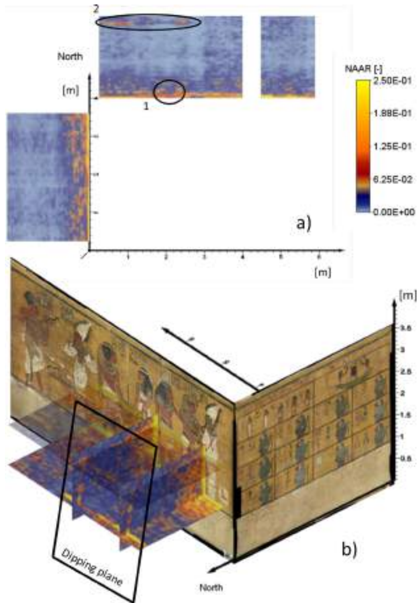
Fig. 4. HF-TM mode processed data: a: Top view of the sections at 1 m from the floor, with evidence of: 1) high amplitude shallow events related to the wall repair and 2) a 2 m deep linear reflection event; b: 3D view of some significant sections: behind the North wall, a clear fracture plane emerges from the combination of vertical and horizontal sections.
