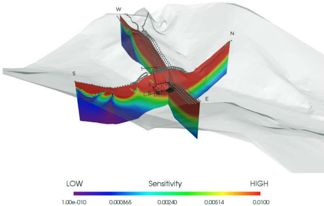
Fig. 5. Sensitivity analysis for the full set of quadrupoles on the KV62 area.
