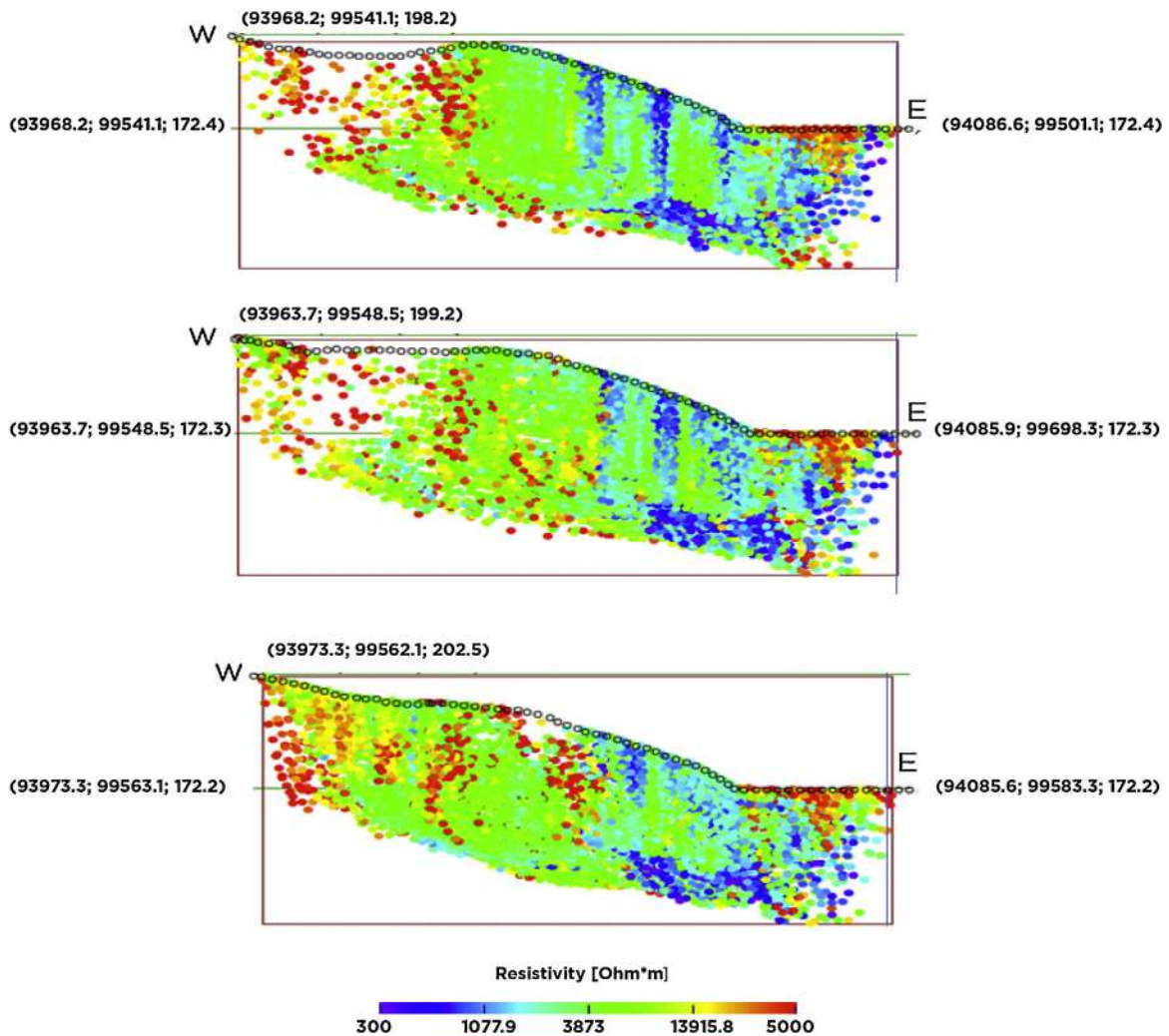
Fig. 4. Apparent resistivity pseudo-plots for electrical resistivity tomography 8 (ERT8), ERT9 and ERT10 after noisy data filtering (from top to bottom).
