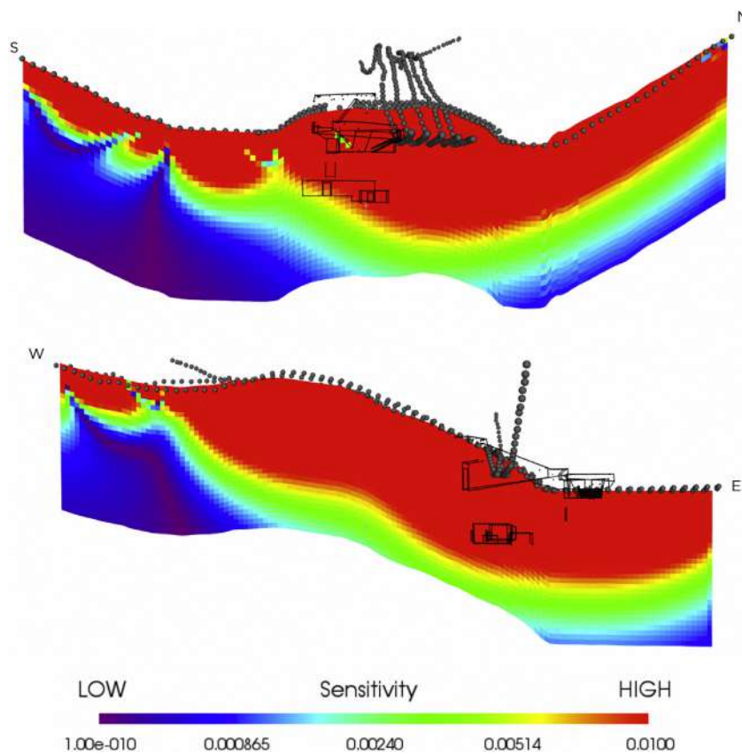
Fig. 6. Sensitivity maps for the full set of quadrupoles on the KV62 area. Top: section below electrical resistivity tomography 13 (ERT13). Bottom: section below ERT10.
