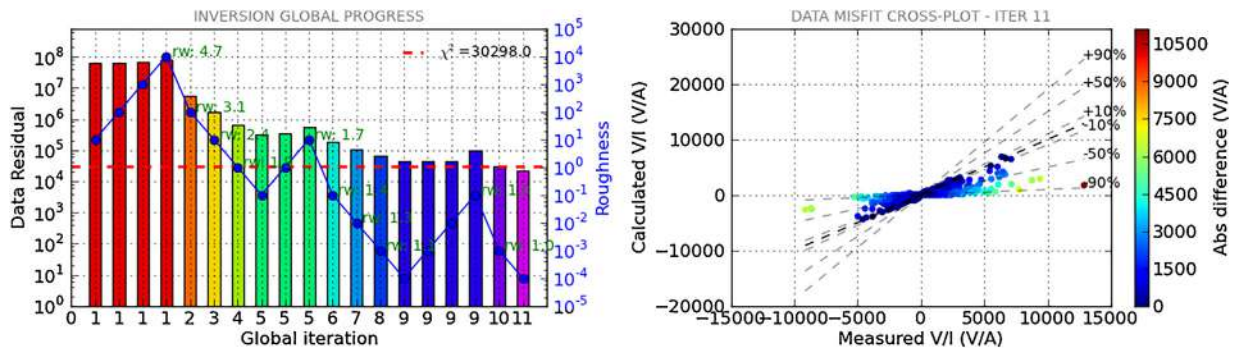
Fig. 7. Inversion progress. Left: data residual and roughness at each iteration trial. Right: cross-plot of measured vs. calculated data.
