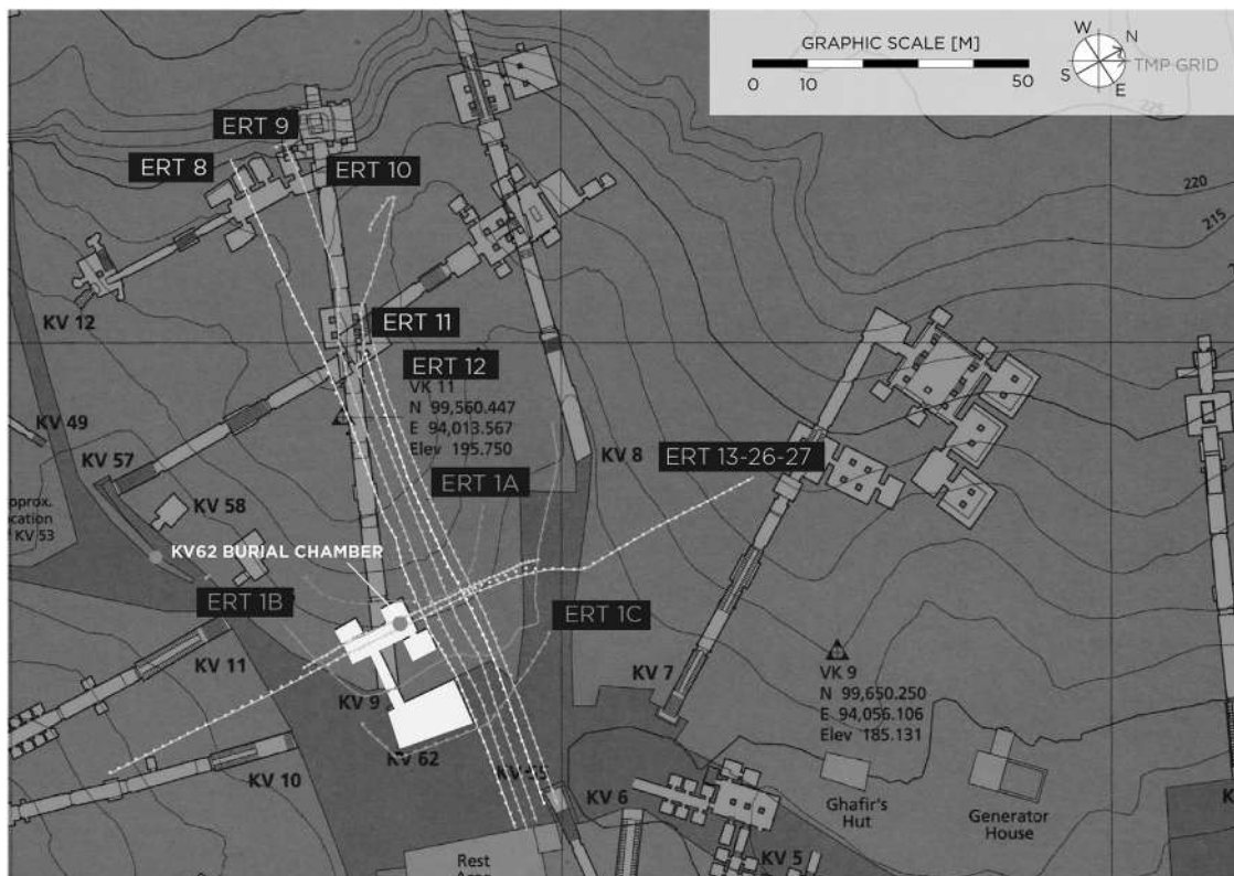
Fig. 1. Detail of the electrical resistivity tomography (ERT) surveys surrounding KV62.
