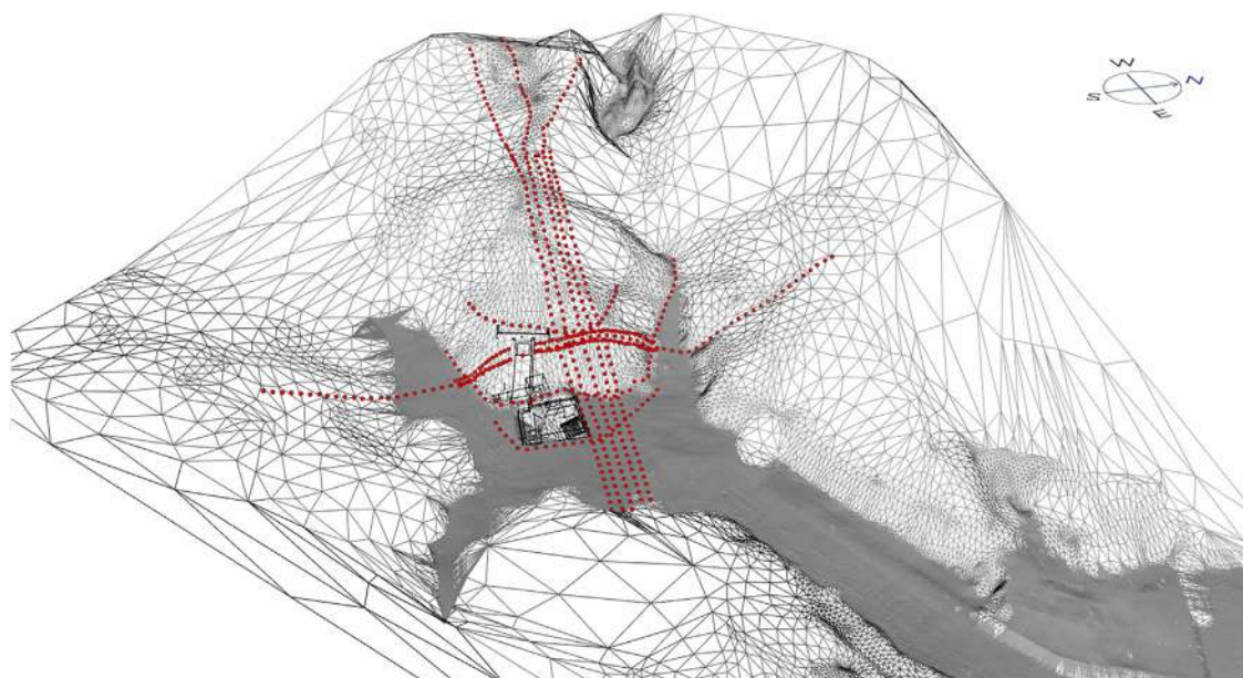
Fig. 3. Topographic survey and electrical resistivity tomography (ERT) lines positions in KV62 area.
