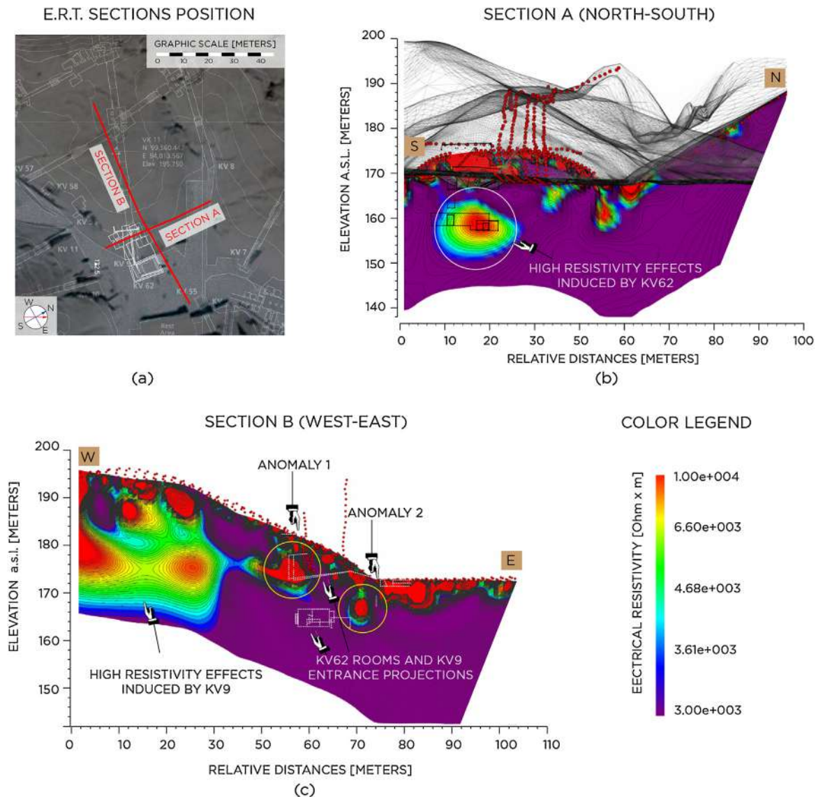
Fig. 9. a: map with the location of vertical electrical resistivity tomography (ERT) sections; b: NS ERT section; c: EW ERT section.
